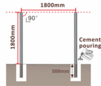
B. Fix the aluminum posts with cement . 500mm under ground
