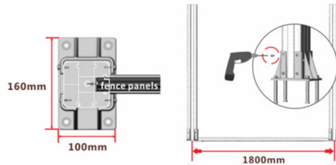
A. Fixing post by using post base
