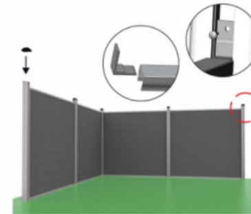
04 Install the top rail and post cap
