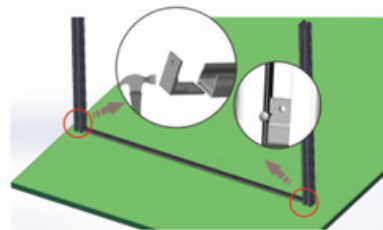
02 Install the bottom rail, using bracket to connect rail with post
